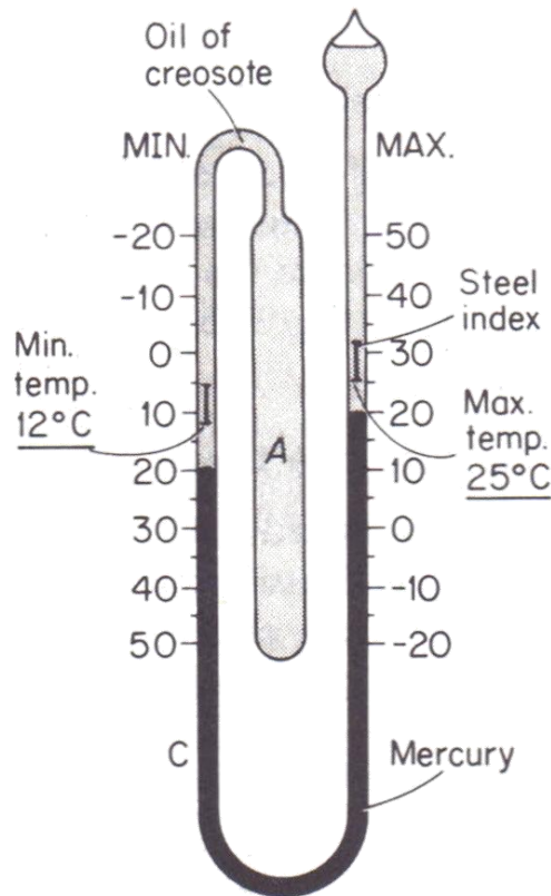
Fig. Six's maximum and minimum thermometer
