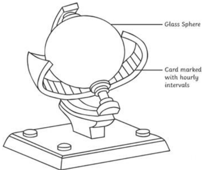
Fig. Sunshine Recorder
